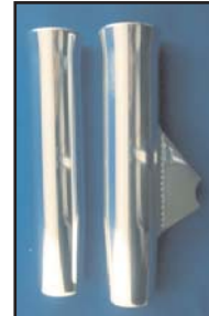
8.5" Swedged with Welded Pins top: without wedge bottom: with wedge
