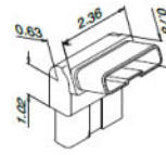
Tap Connector 14.5792.262.00
