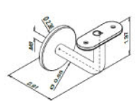
Wall Bracket 14.0111.000.12
