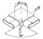
Wall Flange 14.4504.062.12
