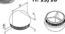
LG Bevel Endcap 14.5730.038.12 H: 13/16"
